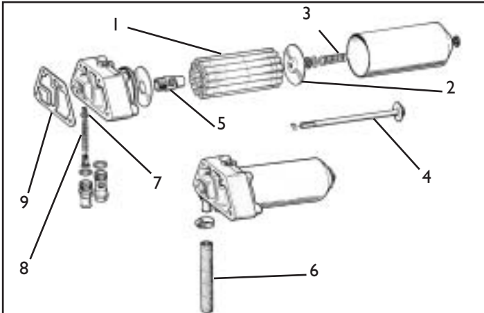
XK Type Engine Cannister Oil Filter
