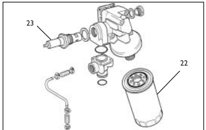
12 Cyl Engine Spin Off Oil Filter
