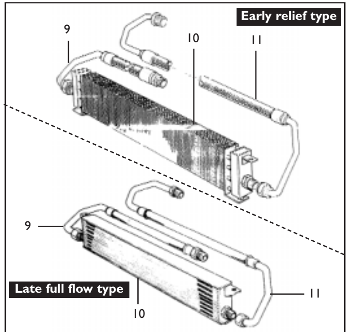
XJS V12/XJ12 Oil Cooler
