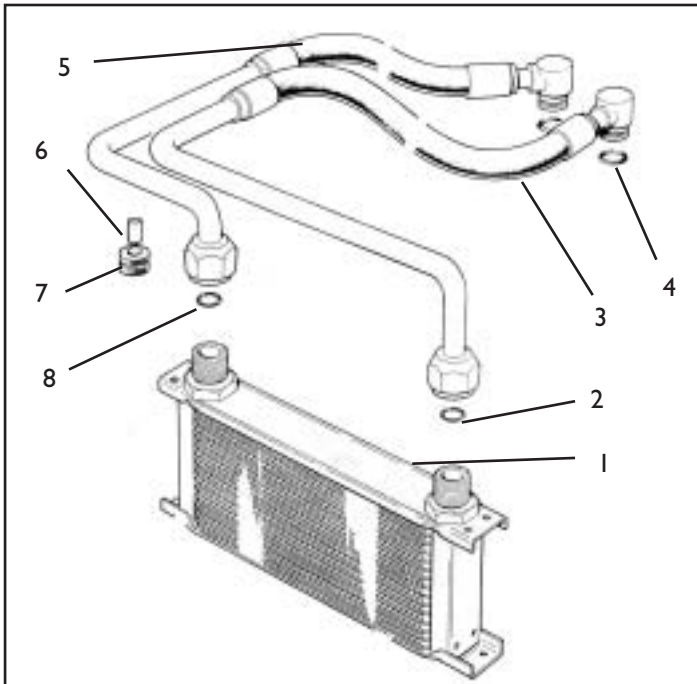
XJ6 Series 3 Oil Cooler
