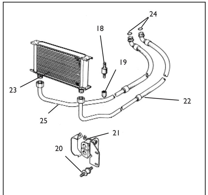
XJS 3.6 Oil Cooler
